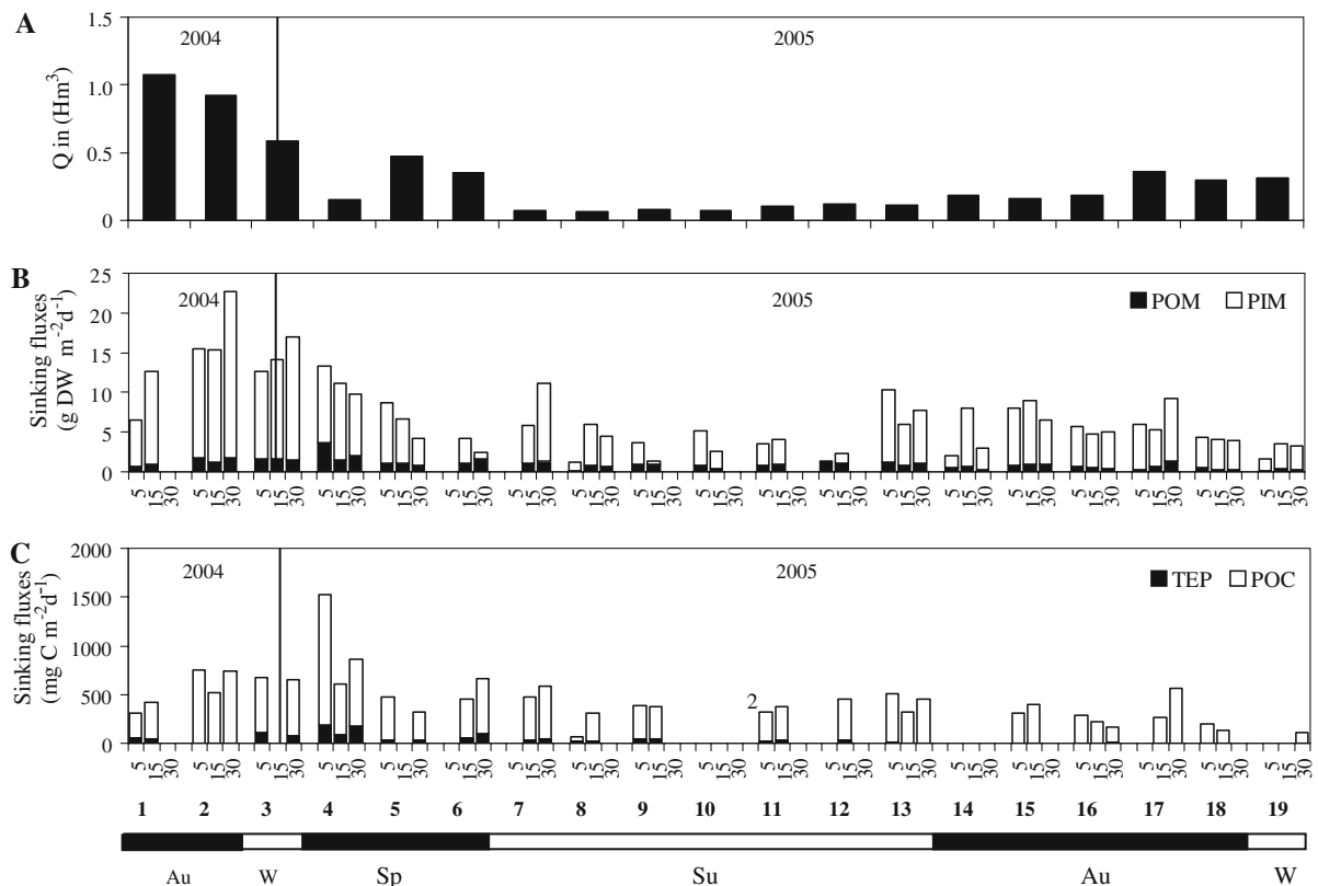
Fig. 3 Seasonal changes in: a water discharge, b sinking fluxes of particulate organic matter (POM) and particulate inorganic matter (PIM) ( \text{g DW m}^{-2} \text{ day}^{-1} ) and c sinking fluxes of particulate organic carbon (POC) and TEP ( \text{mg C m}^{-2} \text{ day}^{-1} ) at 5, 15 and 30 m depths. Note that for avoid any confusion, data for C were removed for those samplings with no data for TEP
